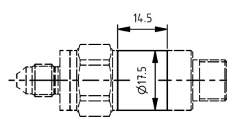
Fig. 9 - Version for voltage output signal (0.5 ... 4.5 VDC)
